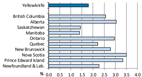
CPI - Fuel Oil And Other Fuels Yellowknife, June 2021 to June 2024
