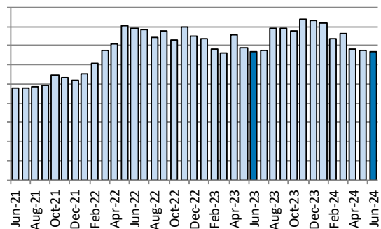
CPI - Fuel Oil And Other Fuels Yellowknife, June 2021 to June 2024
